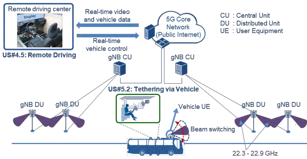
Figure 127: User stories and network architecture of KR TS
