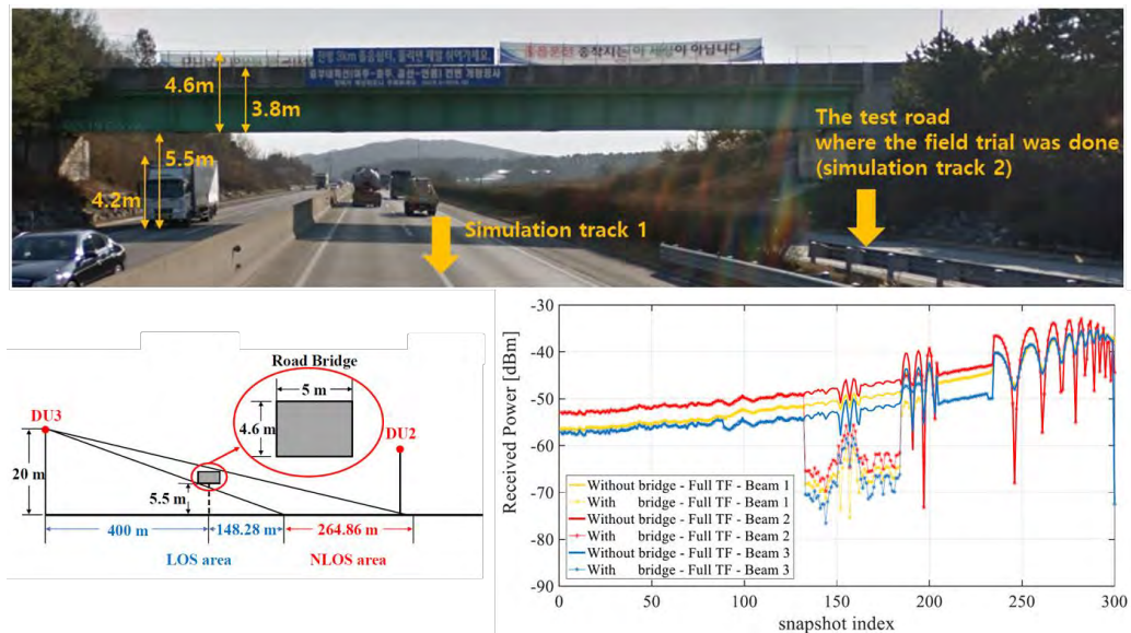
Figure 48: Deployment challenge – signal blockage by a road bridge
