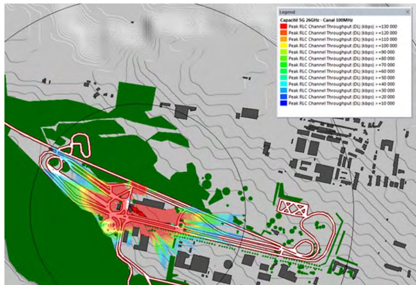
Figure 39: mmWave radio coverage at the Paris-Satory site
