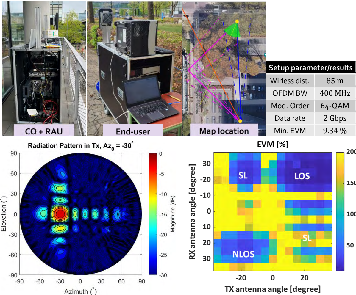
Figure 123: Mm-wave measurements at TU/e. Top: measurement equipment and overview map showing antenna directions and field of view with beamforming as well as setup parameters and main results. Bottom: Antenna radiation pattern and measured EVM across Tx and Rx sc
