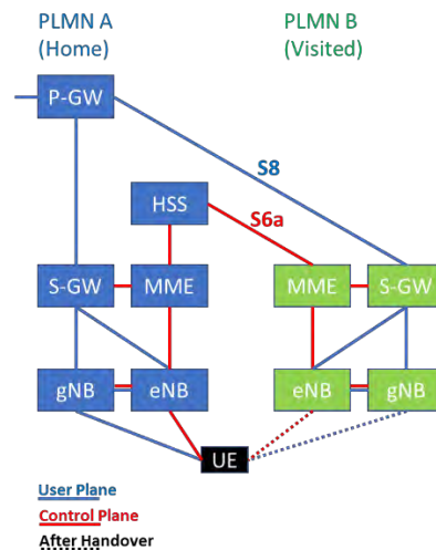
Figure 10: Release with Redirect Architecture without S10 Interface
