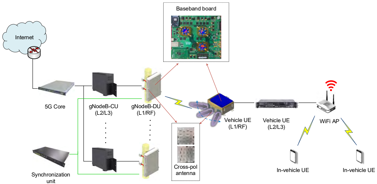
Figure 47: KR trial 5G network setup
