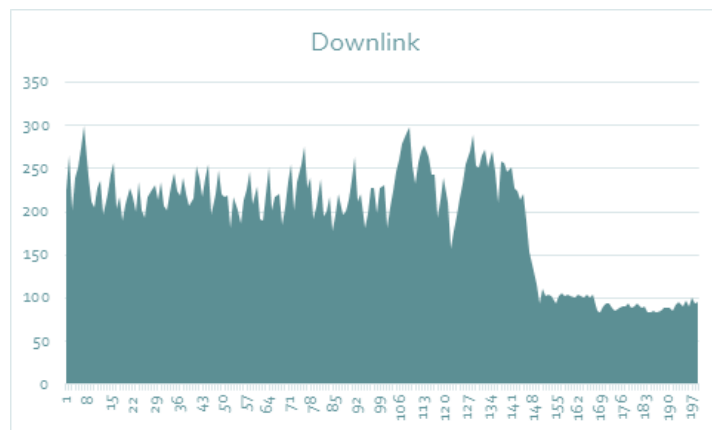
Figure 121: NL TS KPI_AG5 (KPN) DL Throughput Measurement
