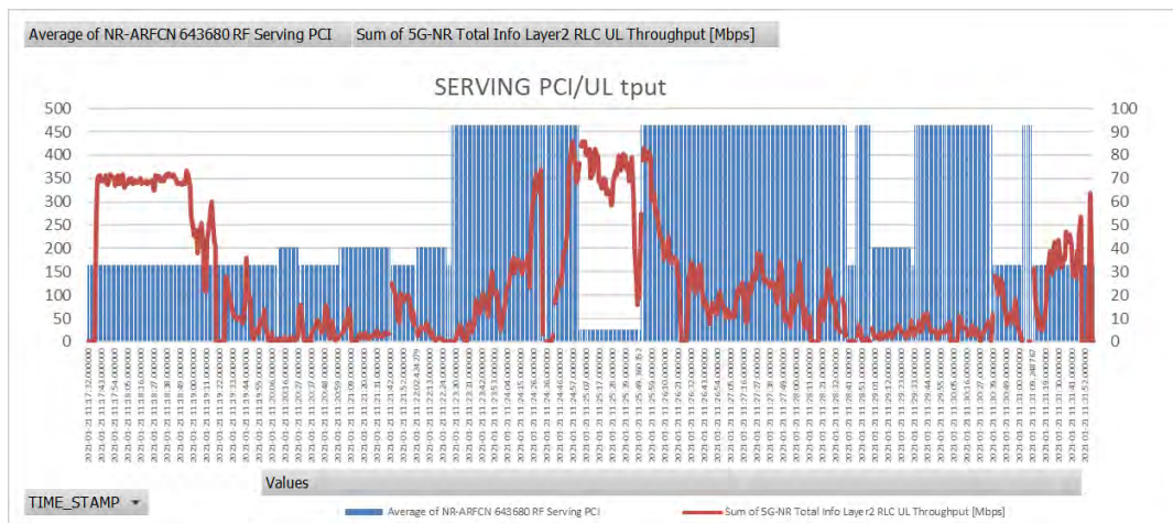
Figure 77: Serving cell and Uplink throughput performance before tuning
