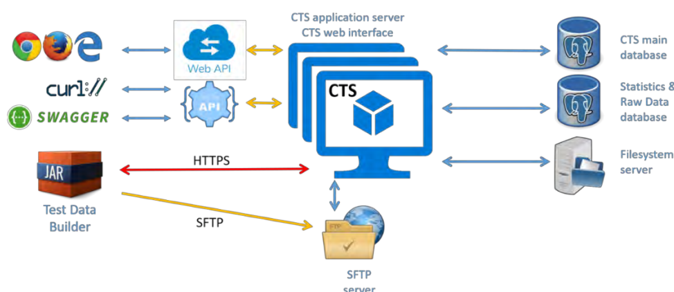
Figure 3: Centralized Test Server architecture
