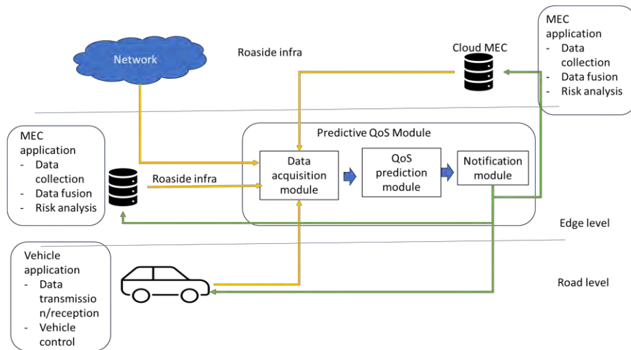
Figure 19: QoS prediction solution
