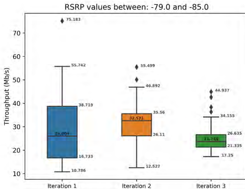
Figure 62: Throughput comparison between three iterations KPI_AG4 DL TCP in New Bridge
