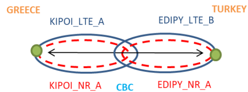
Figure 99: Inter PLMN Handover test setup
