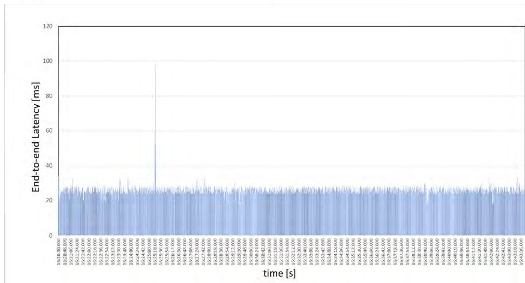
Figure 125: Latency measure in 5G SA network during a UDP DL communication
