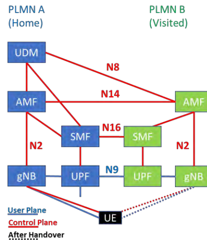
Figure 14: N2 Handover Architecture with Home Routed Roaming (SA)
