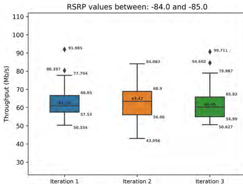
Figure 59: Throughput comparison between three iterations KPI_AG2 UL TCP in Old Bridge
