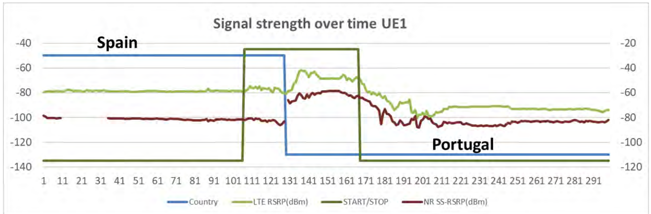
Figure 69: Handover signal strength during verification
