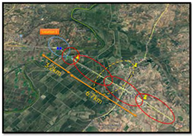
Figure 30: The GR-TR CBC location & layout
