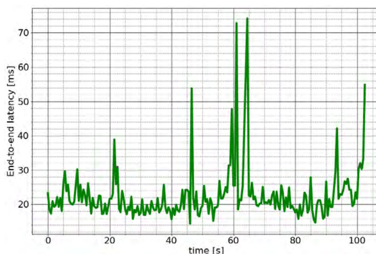
Figure 111: Latency measure in 5G sub 6GHz NSA network during a TCP UL communication
