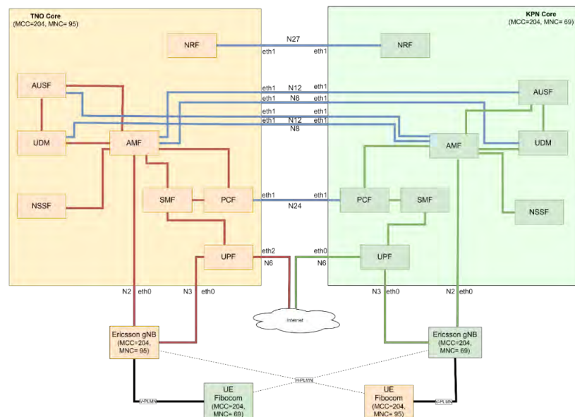
Figure 43: NL TS Roaming Implementation
