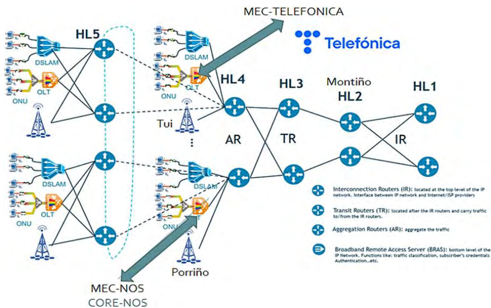
Figure 28: Distributed Cores and MECs Interconnection
