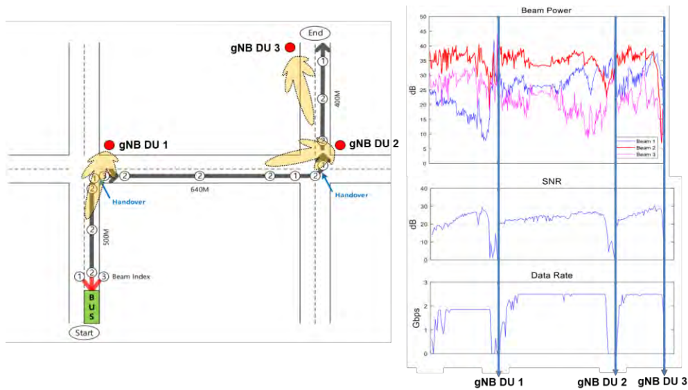
Figure 130: Measured receive SNR and downlink data rate of PHY-to-PHY testing in Daejeon city, south Korea
