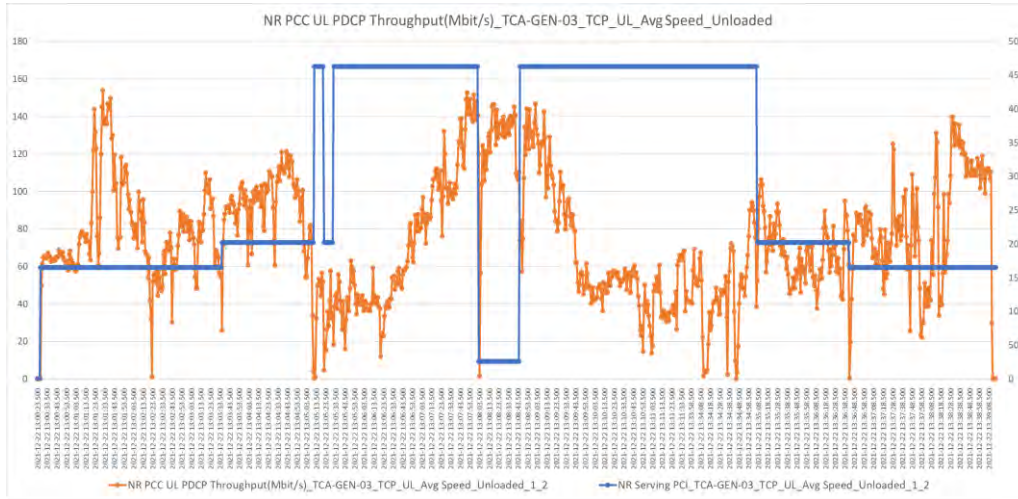
Figure 78: Serving cell and Uplink throughput performance after tuning
