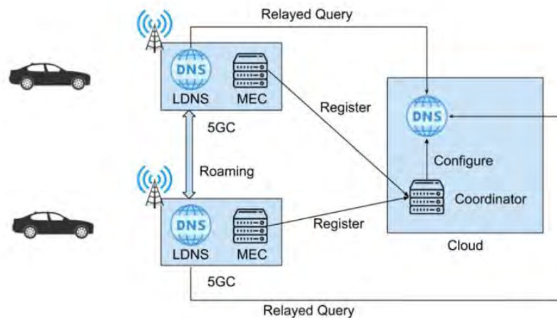
Figure 17: Architecture for Continuity Measures
