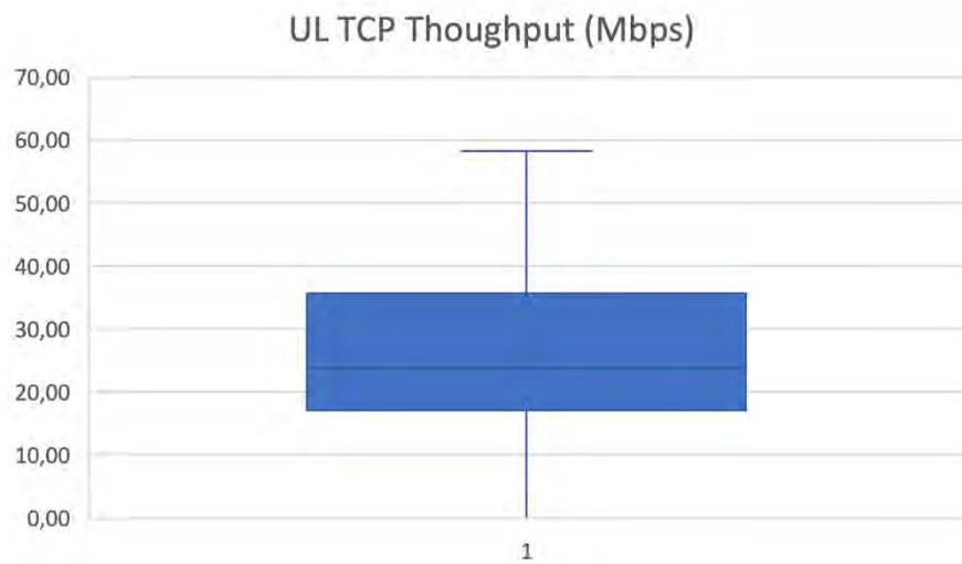
Figure 104: UL TCP Throughput with good conditions - O2 SIM
