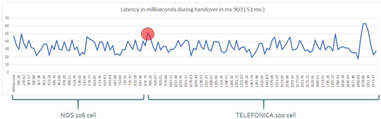
Figure 68: NOS 106 cell to TELEFONICA 100 cell handover latency
