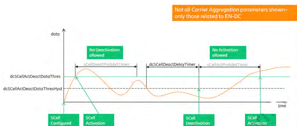
Figure 83: LTE-NR Downlink and Uplink CA parameters working mechanism
