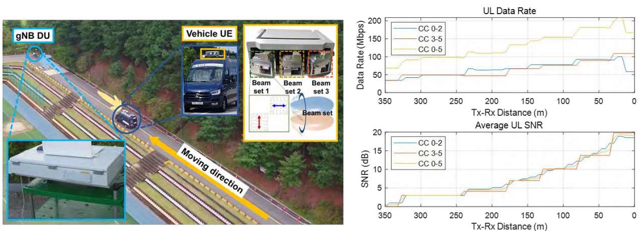
Figure 129: Measured receive SNR and uplink data rate of PHY-to-PHY testing in ETRI premises, south Korea
