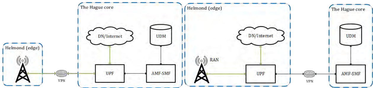
Figure 117: NL TS Core Routing (Left) and LBO Routing (Right) Setup (Edge-Core Network)
