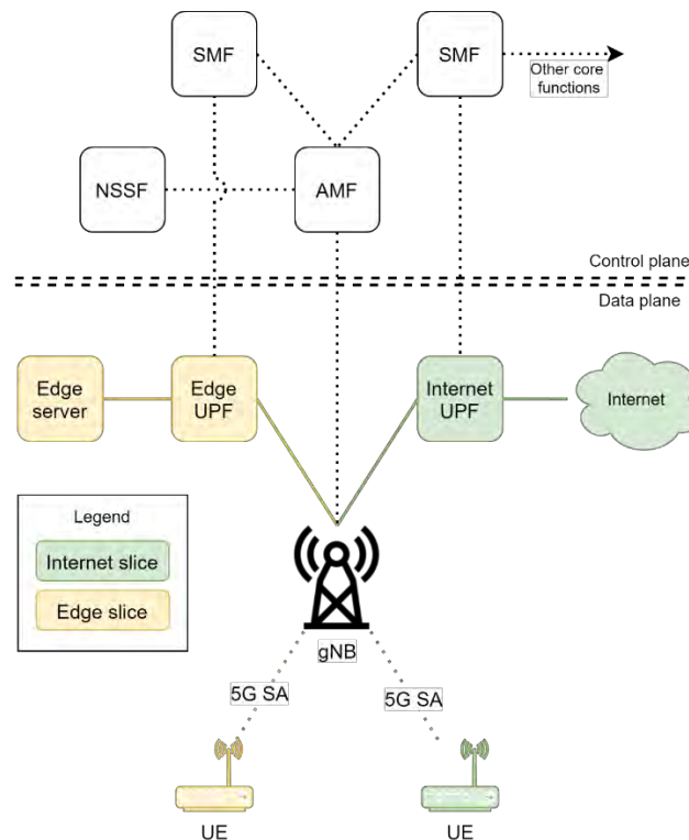
Figure 18: Slicing in RAN and core network in combination with local breakout and edge computing
