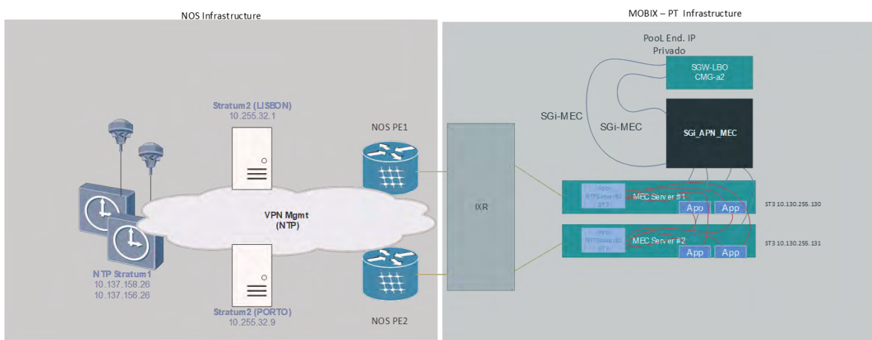
Figure 52: Time synchronization architecture for the PT MEC server applications
