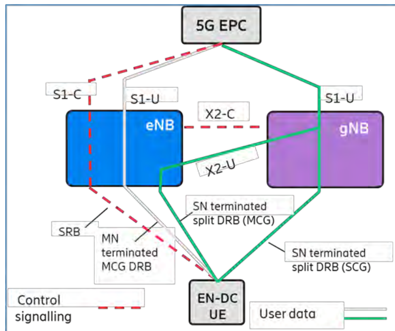
Figure 31: NR NSA Option 3x Architecture
