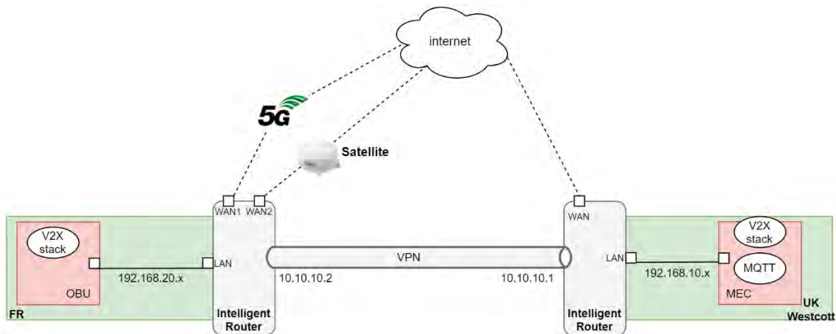
Figure 20: Hybrid 5G-satellite intelligent routing-based deployment at the French test site
