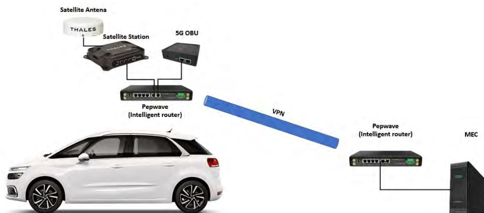
Figure 41: Satellite connectivity scenario
