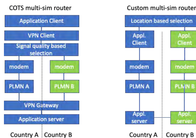
Figure 15: Comparing COTS and custom multi-sim router
