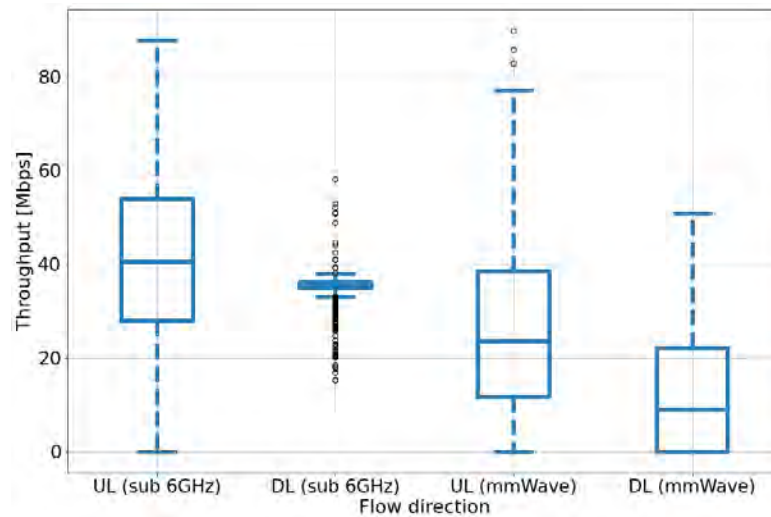
Figure 112: Throughput distribution for different flow direction with sub 6GHz and mmWave 5G NSA networks
