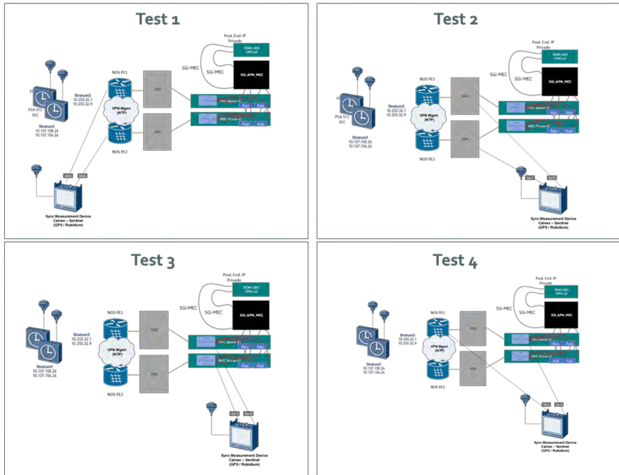
Figure 54: Time synchronization accuracy tests performed at the NOS network
