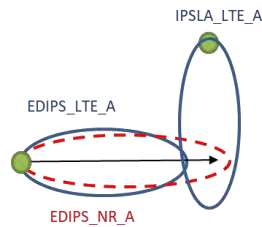
Figure 97: Inter-MeNB handover without SgNB change triggered by MeNB test setup
