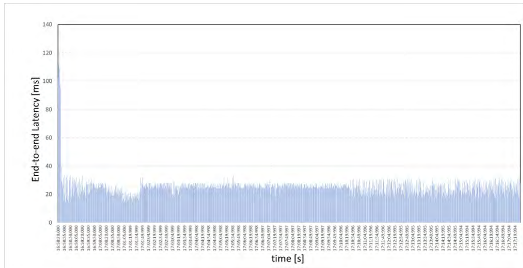
Figure 126: Latency measure in 5G SA network during a TCP DL communication
