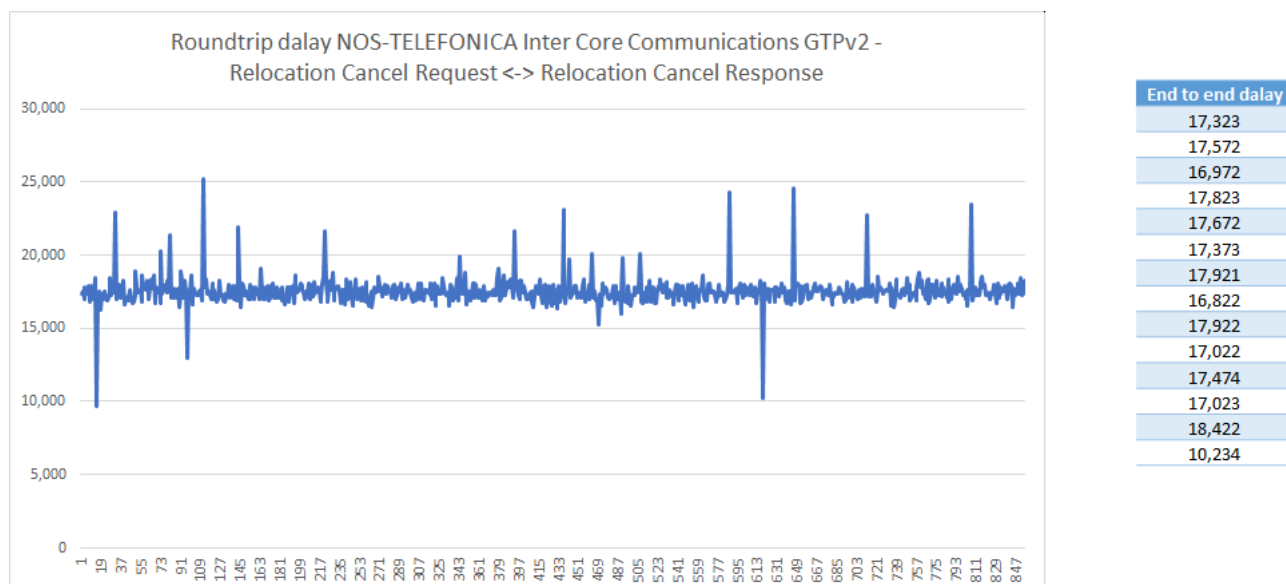
Figure 63: Roundtrip delay NOS-TELEFONICA Inter Core Communications
