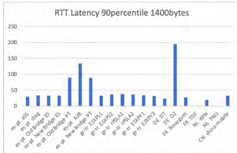
Figure 9: Round trip latency 1400 bytes 90percentile
