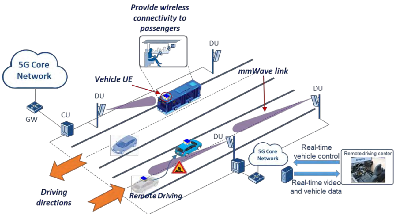
Figure 46: KR network layout for Tethering via Vehicle and Remote Control Driving
