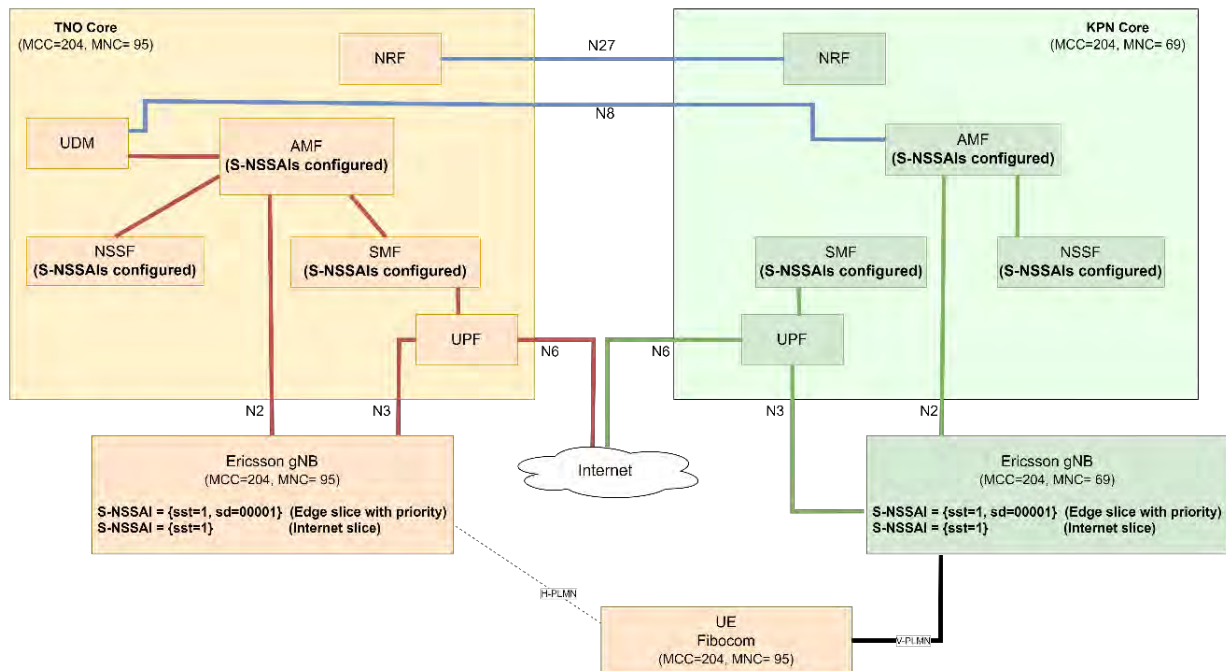
Figure 44: NL TS Roaming with slicing implementation
