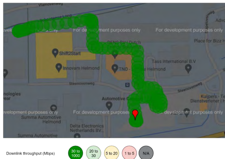
Figure 122: NL TS KPI_AG5 (KPN) DL Throughput Measurement
