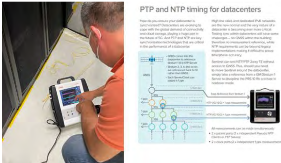
Figure 53: Calnex Sentinel equipment for time synchronization measurements
