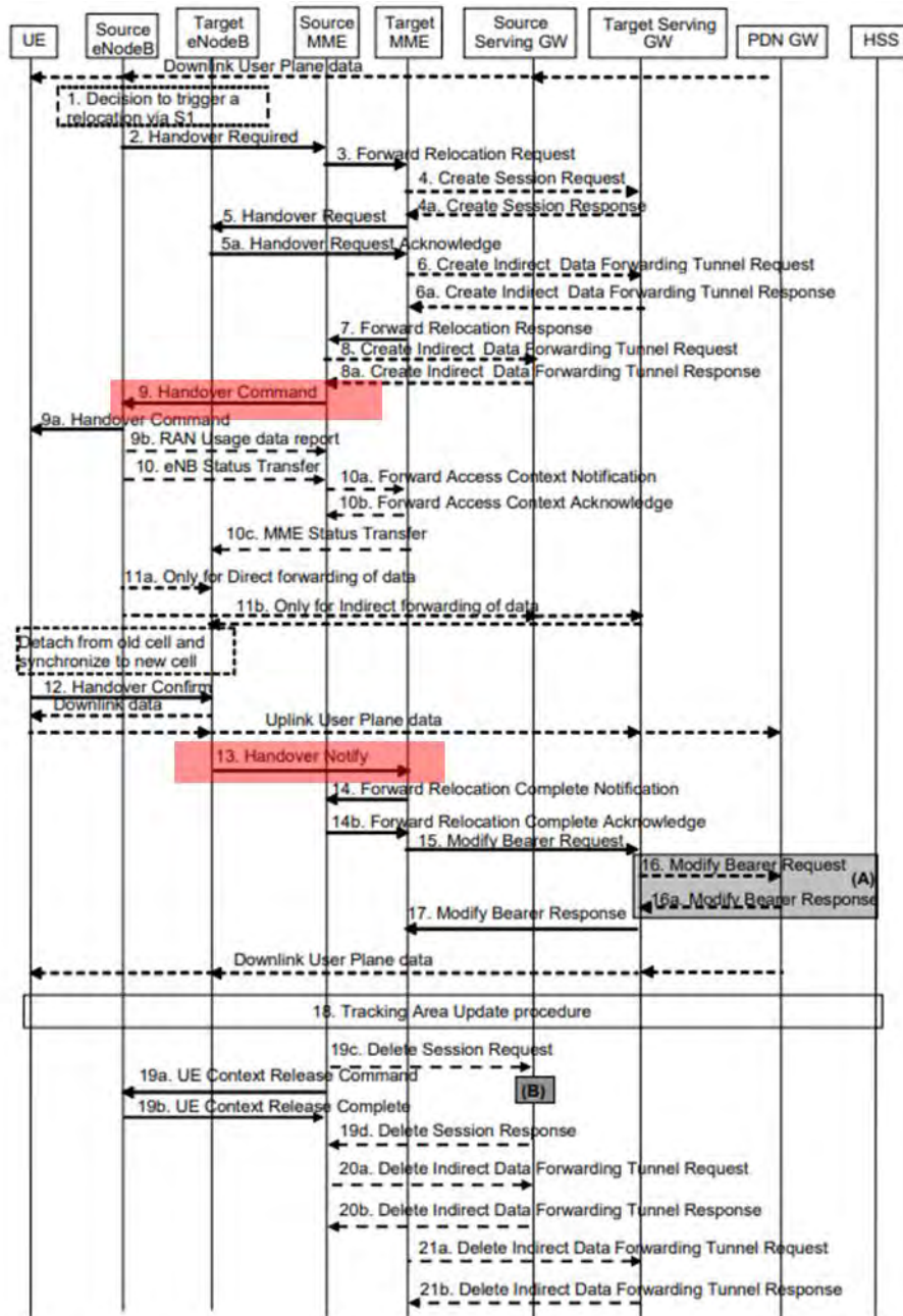
Figure 100: Inter MME Handover signaling flow (3GPP TS 23.401)
