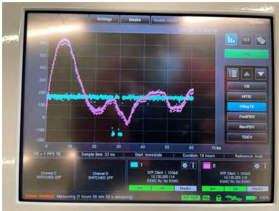
Figure 56: Time synchronization measurements obtained at the PT MEC
