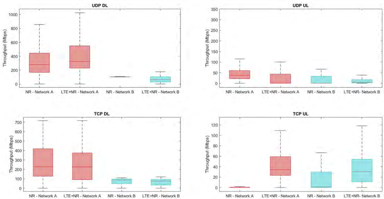
Figure 108: Drive test throughput results (TCP and UDP) for the two networks utilized in the specific trials in FI-TS
