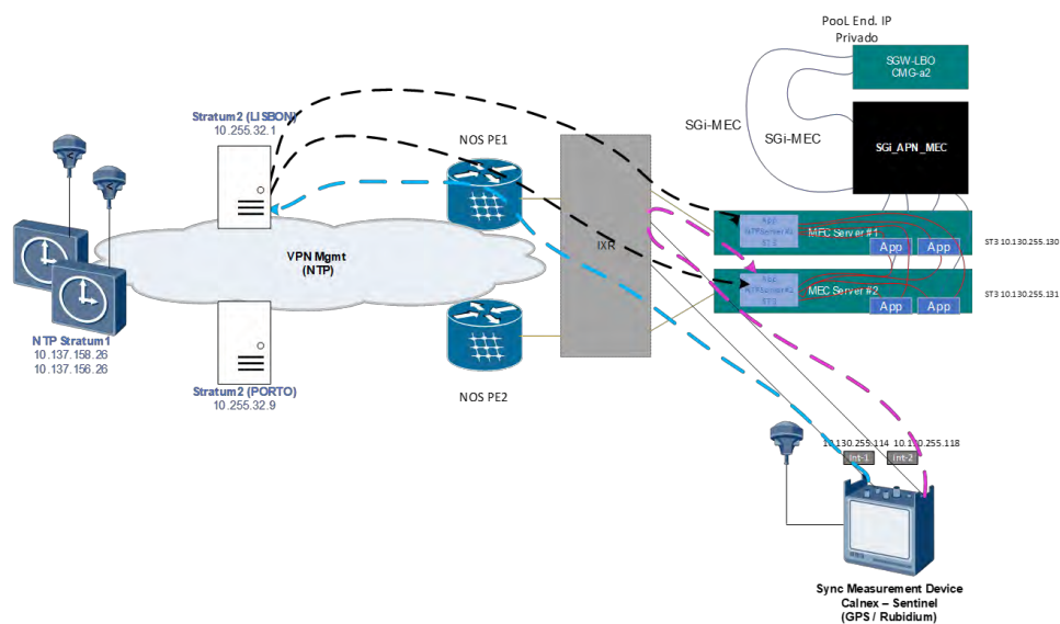
Figure 54: Time synchronization accuracy tests performed at the NOS network
