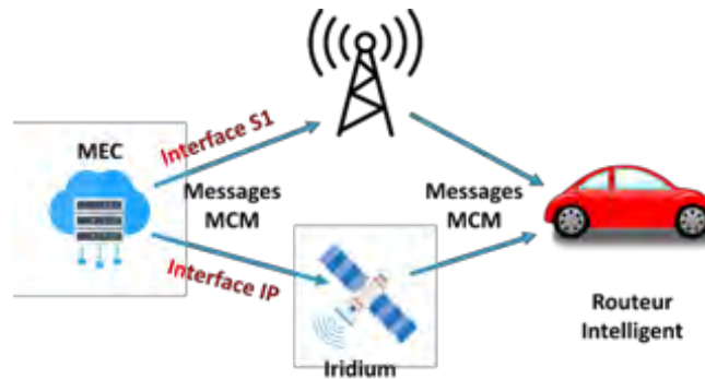
Figure 40: Satellite connectivity architecture
