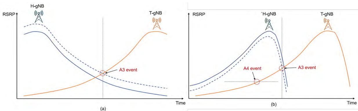
Figure 25: RSRP distribution during handover: a) Conventional omni- or bi-directional gNodeB deployment; b) Uni-directional gNodeB deployment
