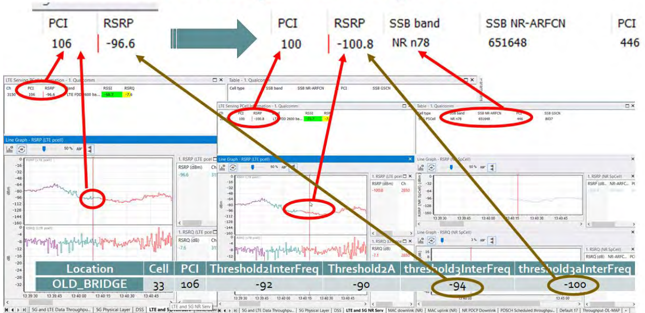
Figure 65: Handover from 4G NOS to 5G TEF
