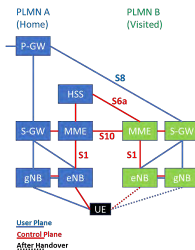
Figure 13: S1 Handover Architecture with Home Routed Roaming (NSA)
