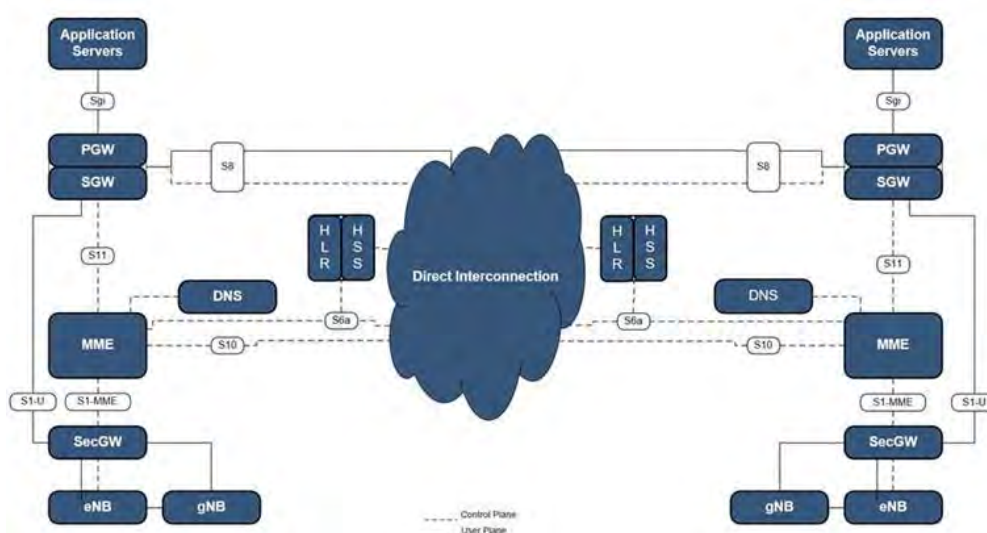
Figure 73: Overall Architecture Interconnection between Turkcell and Cosmote
