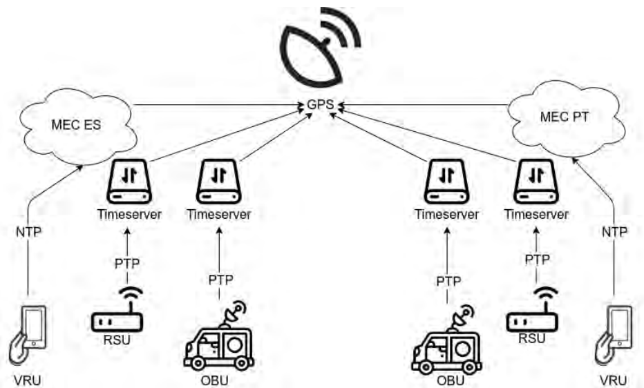
Figure 49: General view of time synchronization approach in ES-PT CBC
