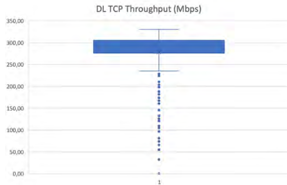
Figure 101: DL TCP Throughput with good conditions - DT SIM
