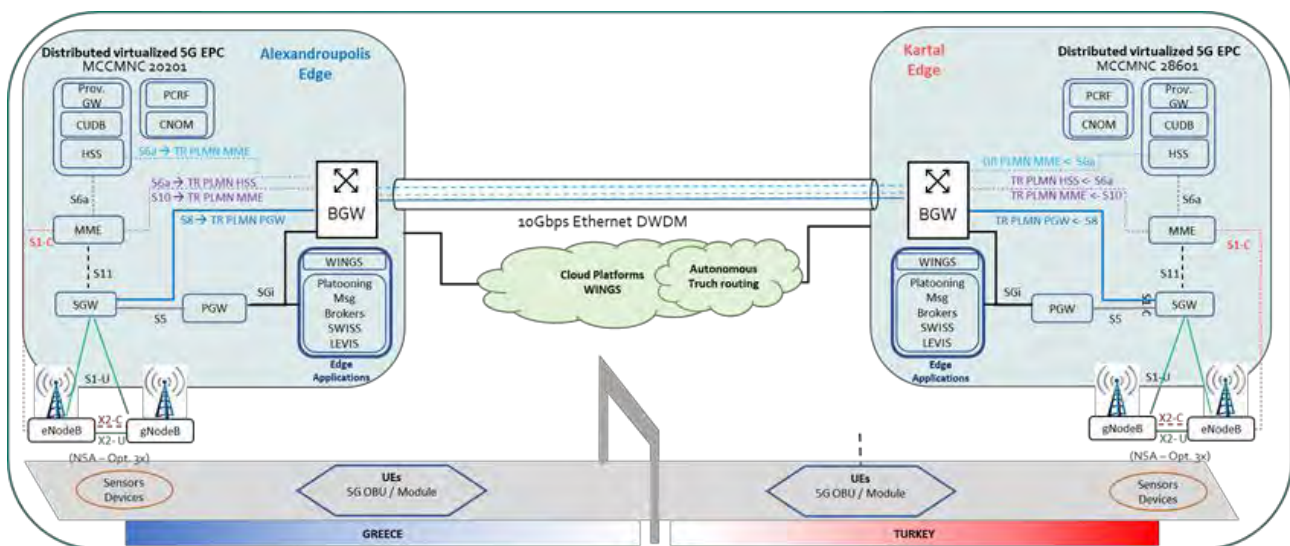
Figure 32: Overall Architecture
