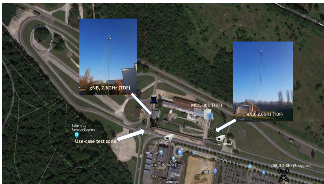
Figure 109: A 5G mmWave network has been deployed at Satory
