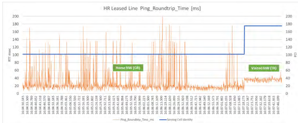
Figure 91: HR configuration - leased line connection RTT performance
