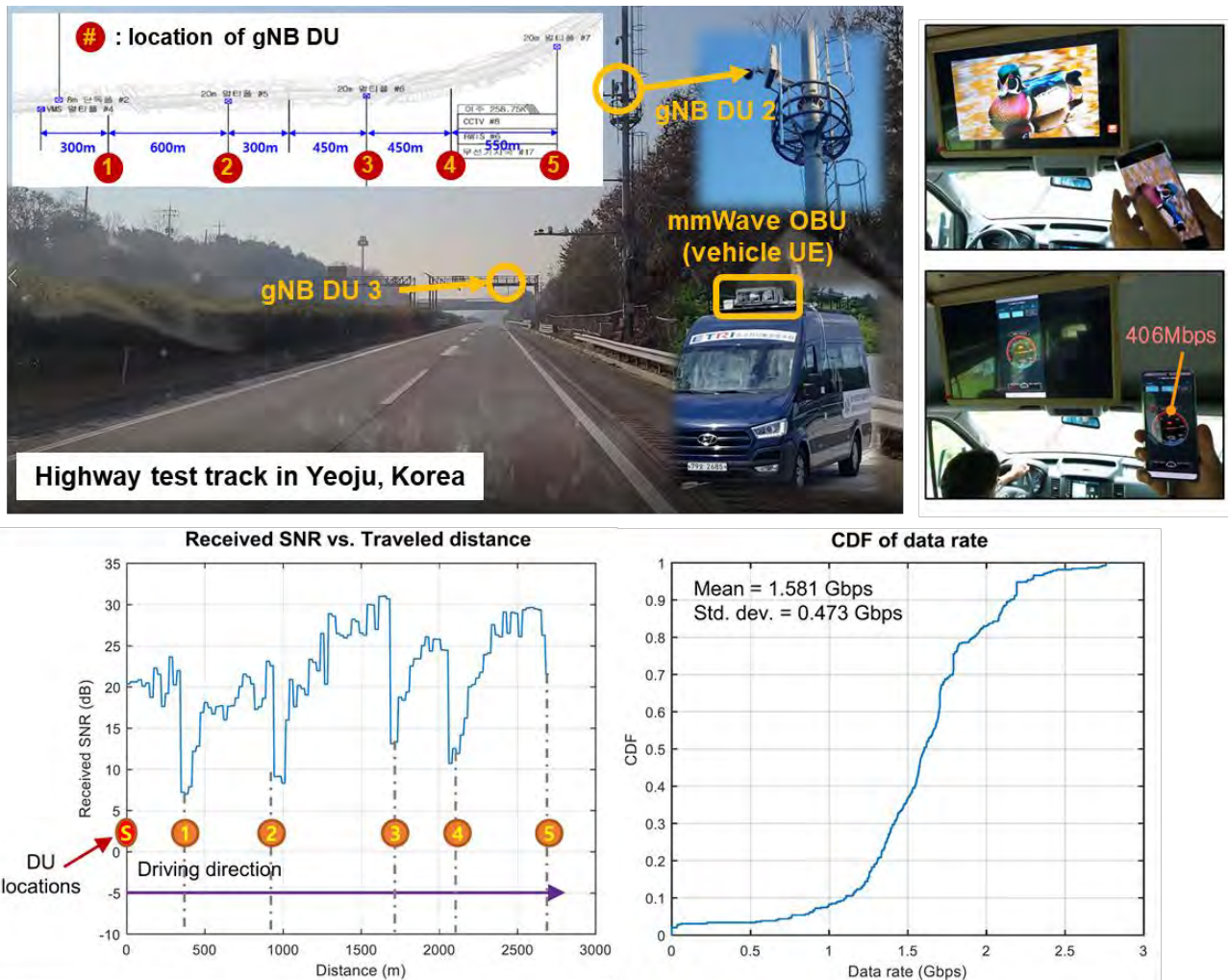
Figure 131: Field trial conducted on a highway test track in Yeosu, Korea
