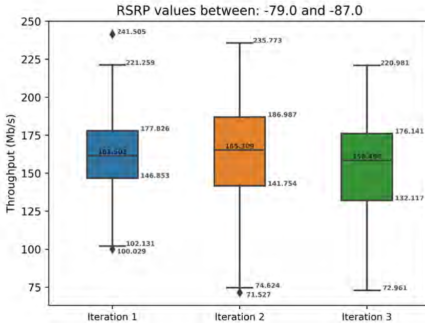
Figure 60: Throughput comparison between three iterations KPI_AG3 DL TCP in New Bridge
