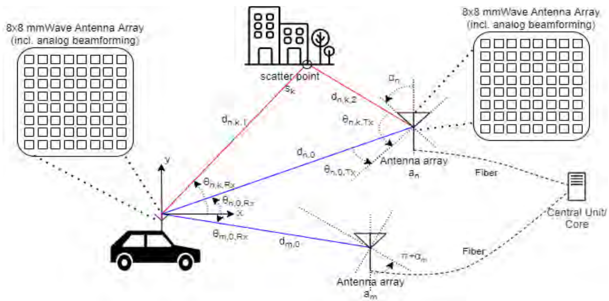
Figure 23: Architecture and setup schematic for precise positioning using compressed sensing and angular information from 5G mmWave signals
