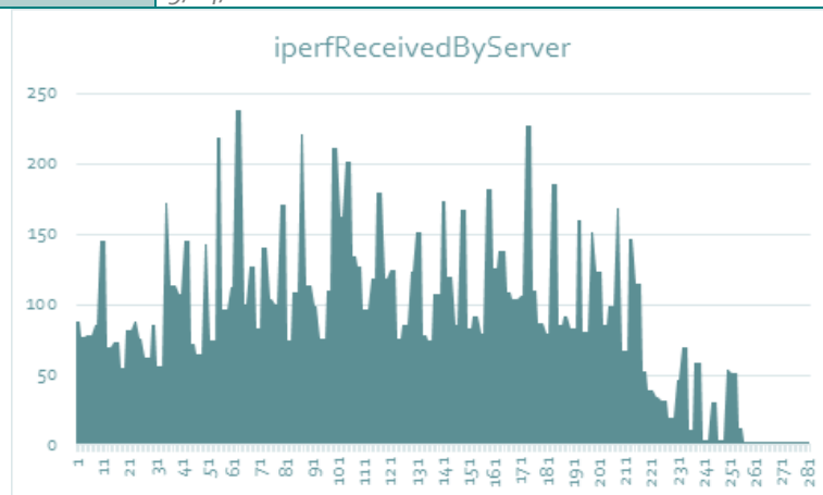
Figure 119: NL TS KPI_AG5 (TNO) DL Throughput Measurement
