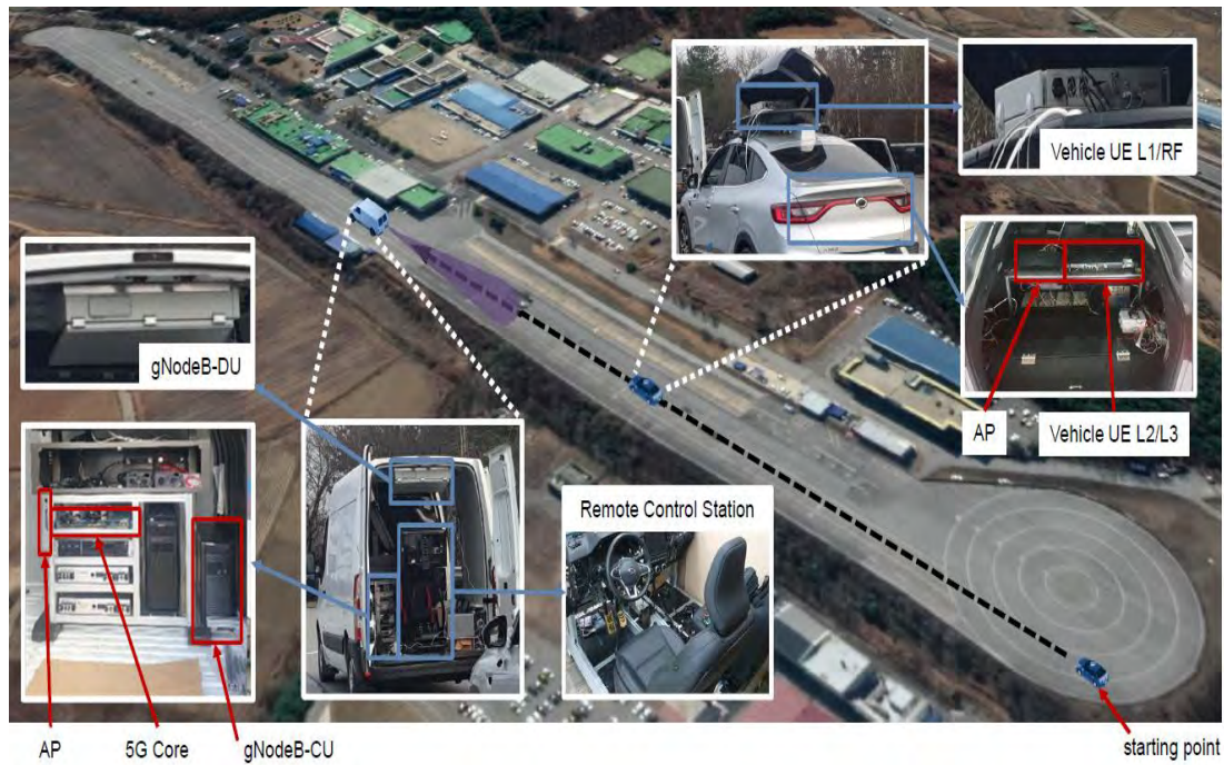
Figure 128: Remote control test setup and testing in KATECH proving ground, South Korea
