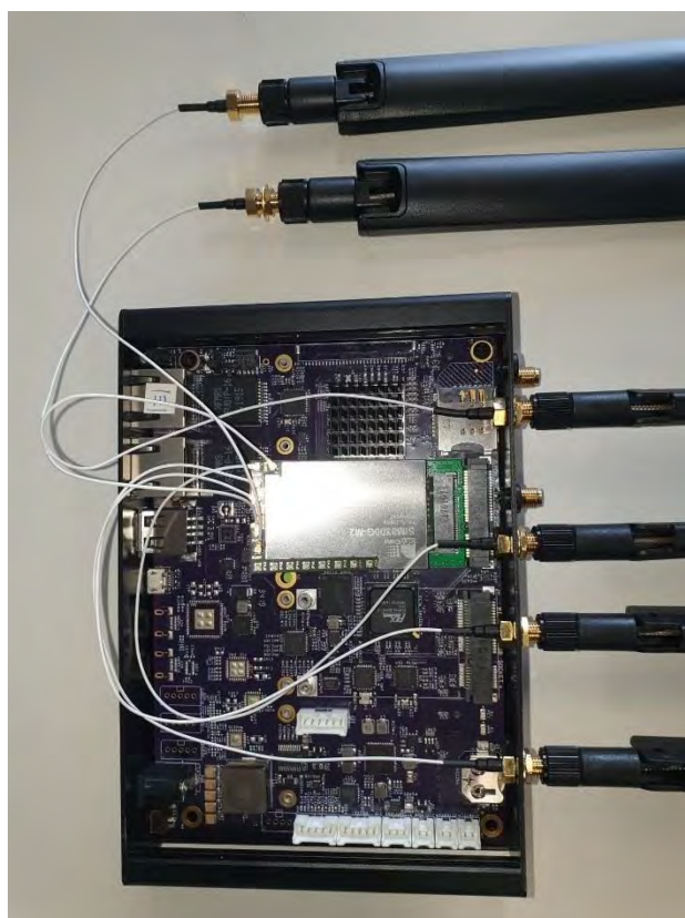
Figure 110: 5G mmWave OBU
