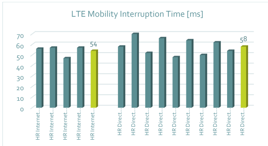
Figure 93: LTE Mobility Interruption time [ms]
