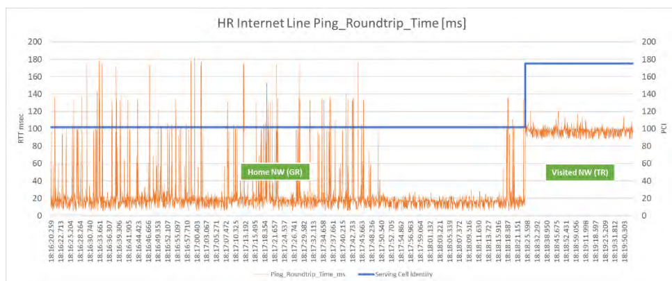
Figure 90: HR configuration - internet connection RTT performance
