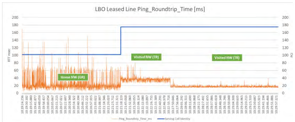
Figure 92: LBO configuration - leased line connection RTT performance
