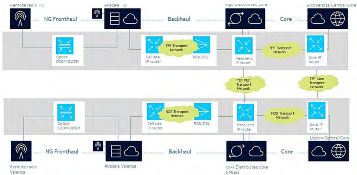
Figure 26: Telefónica & NOS Network architecture
