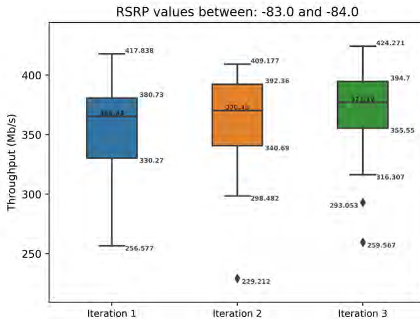
Figure 57: Throughput comparison between three iterations KPI_AG1 DL TCP in Old Bridge
