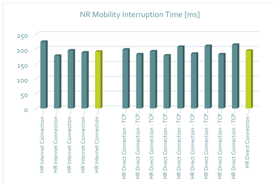
Figure 94: NR Mobility Interruption time [ms]
